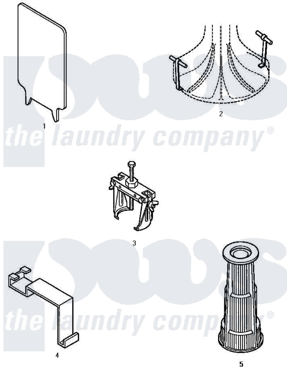
Amana Residential Amana LW9203W (BOM: P1163401W W) Washer Parts Parts Diagram 17 - SPECIAL TOOLS
