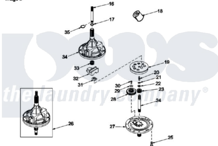
Amana Residential Amana LWA65AL (BOM: PLWA65AL) Washer Parts Parts Diagram 02 - BEARINGS, BRAKE & PULLEY & TRANSMISSION
