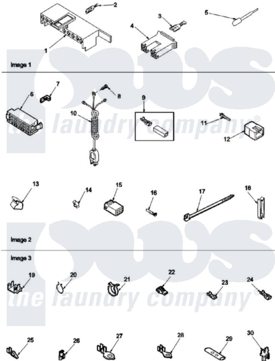
Amana Residential Amana LWA65AW (BOM: PLWA65AW) Washer Parts Parts Diagram 04 - CONNECTION BLOCKS, EXTRACTOR TOOL
