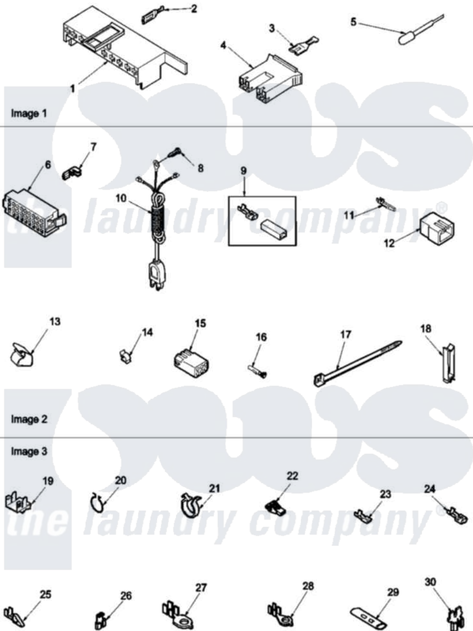
Amana Residential Amana LWA90AL (BOM: PLWA90AL) Washer Parts Parts Diagram 04 - CONNECTION BLOCKS AND EXTRACTOR TOOL Click on the part number to view part
