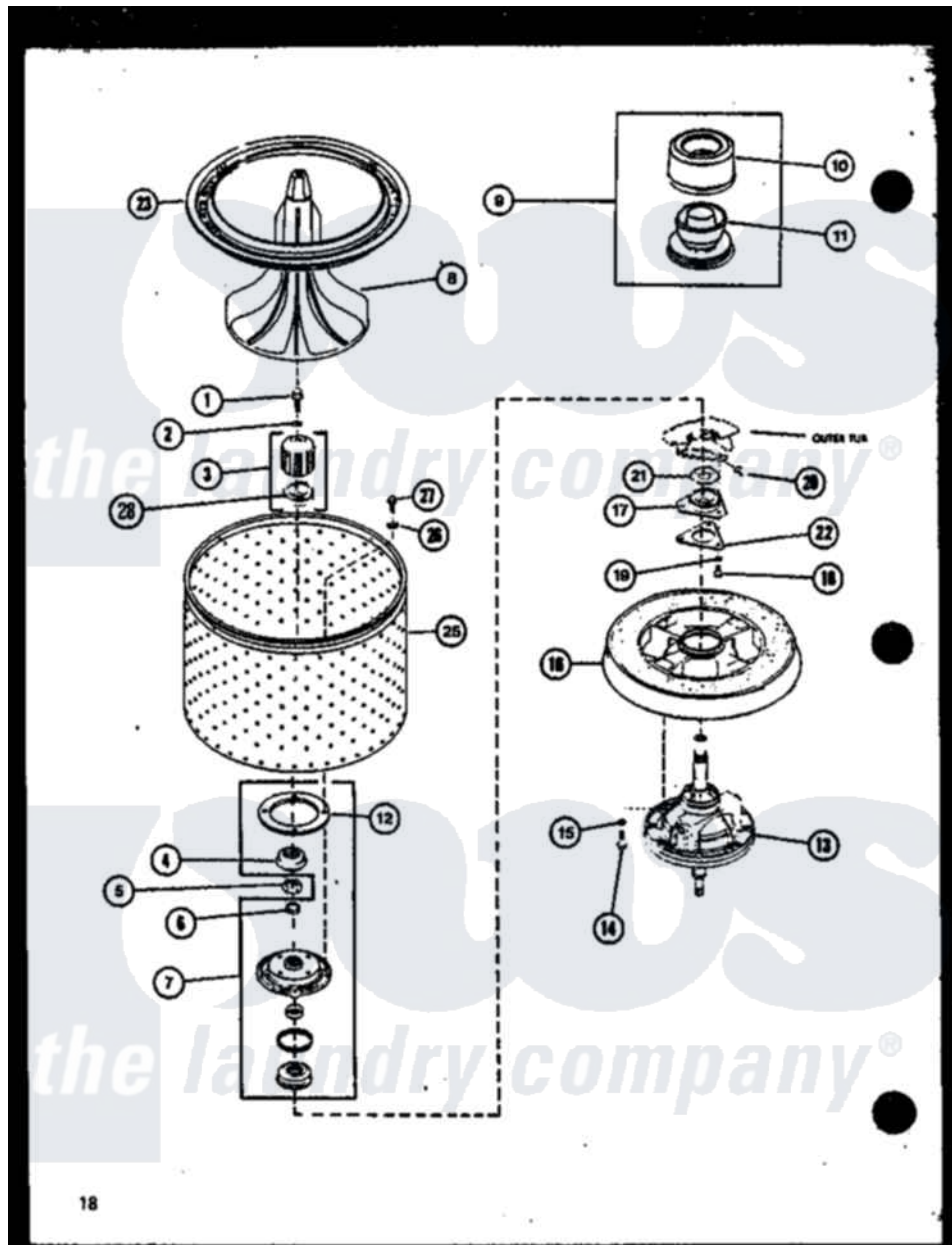
Amana Residential Amana LWD250 (BOM: P7762128W W) Washer Parts Parts Diagram 06 - Page 7 Click on the part number to view part
