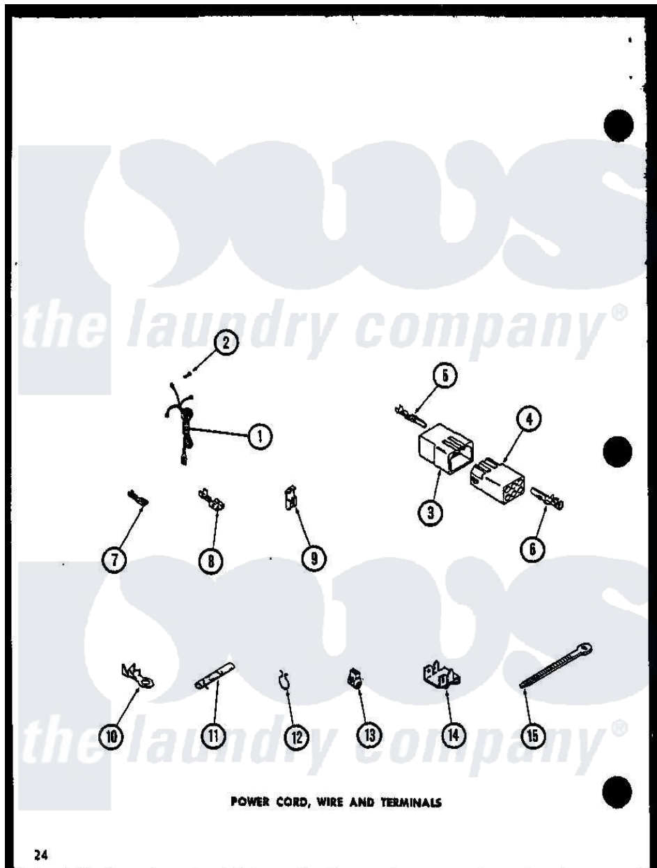
Amana Residential Amana LWD352 (BOM: P1110507W W) Washer Parts Parts Diagram 08 - POWER CORD Click on the part number to view part
