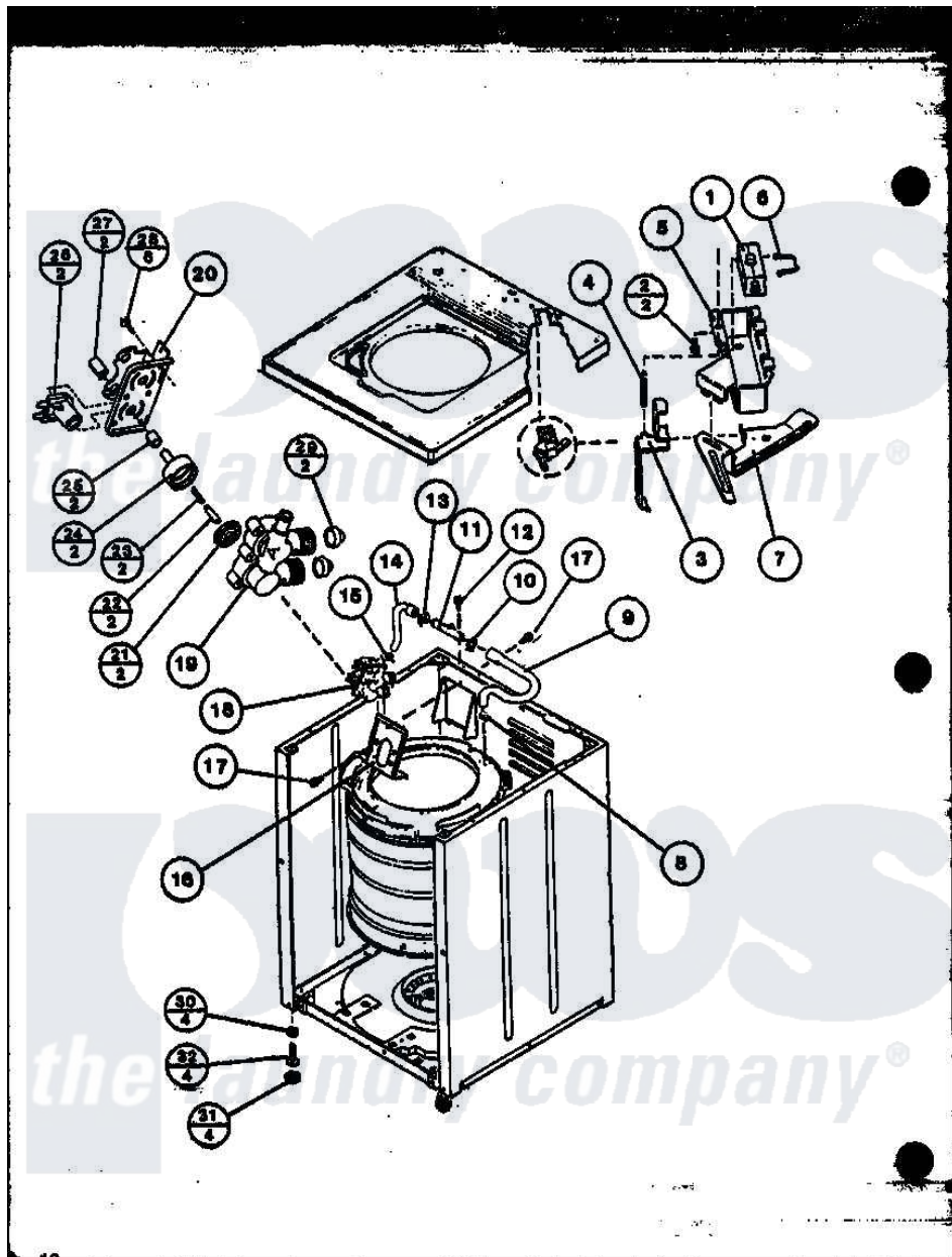
Amana Residential Amana LWD352L (BOM: P1122911W L) Washer Parts Diagram 02 - Page 4 Click on the part number to view part
