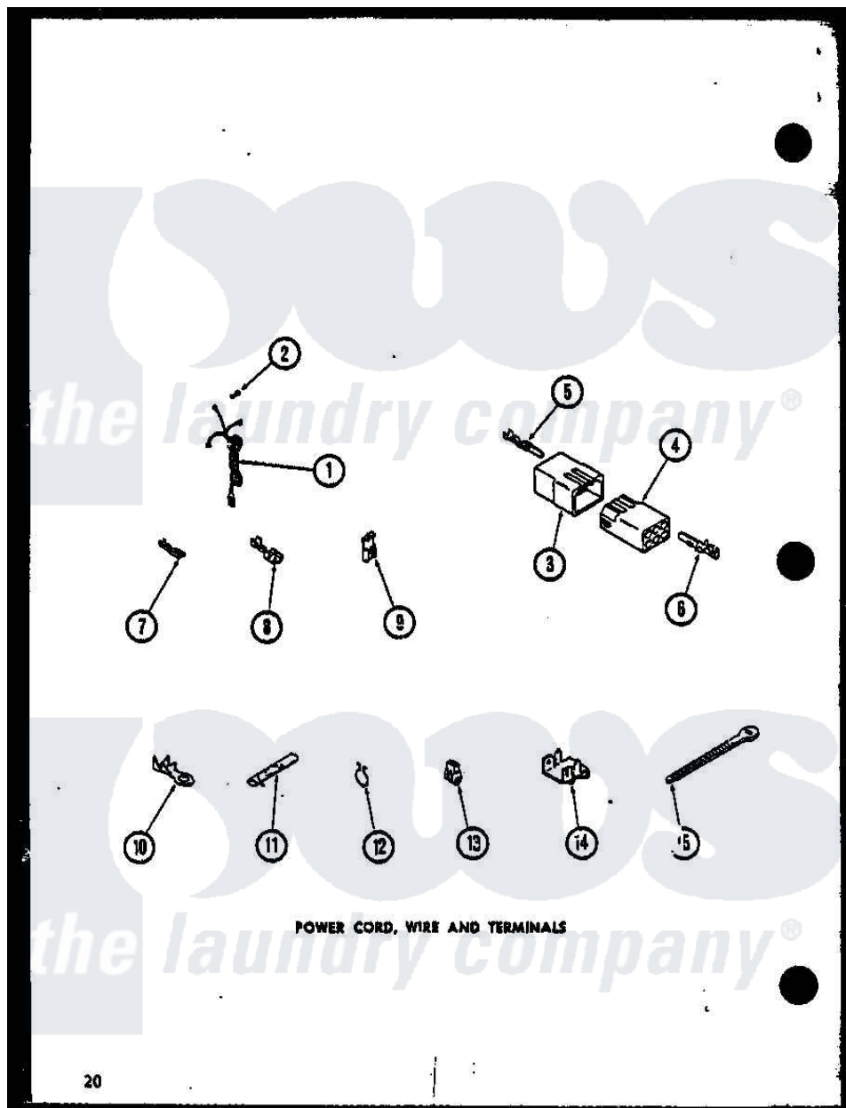
Amana Residential Amana LWD352W (BOM: P1122913W) Washer Parts Parts Diagram 06 - POWER CORD
