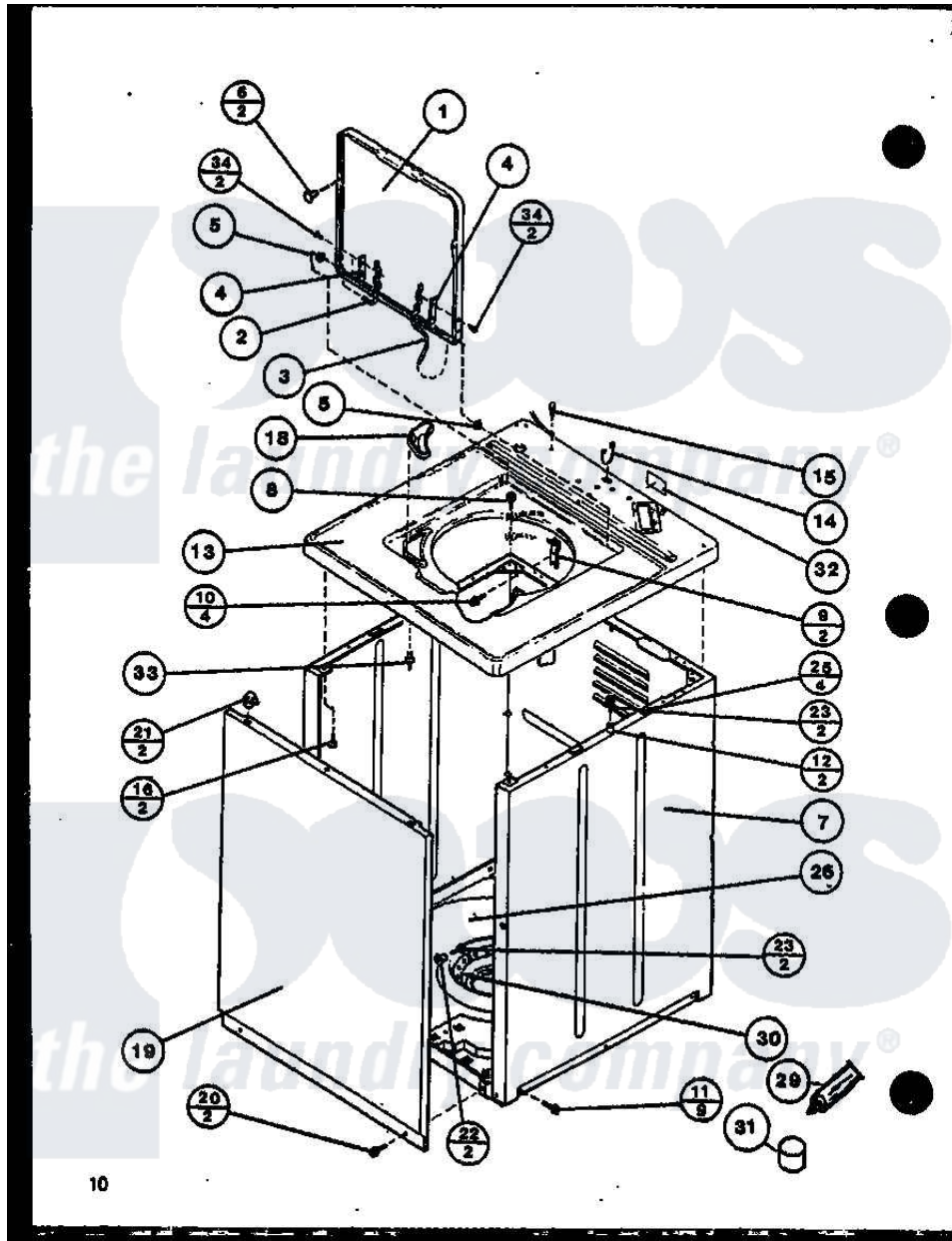
Amana Residential Amana LWD353L (BOM: P1122916W) Washer Parts Parts Diagram 01 - Page 3 Click on the part number to view part
