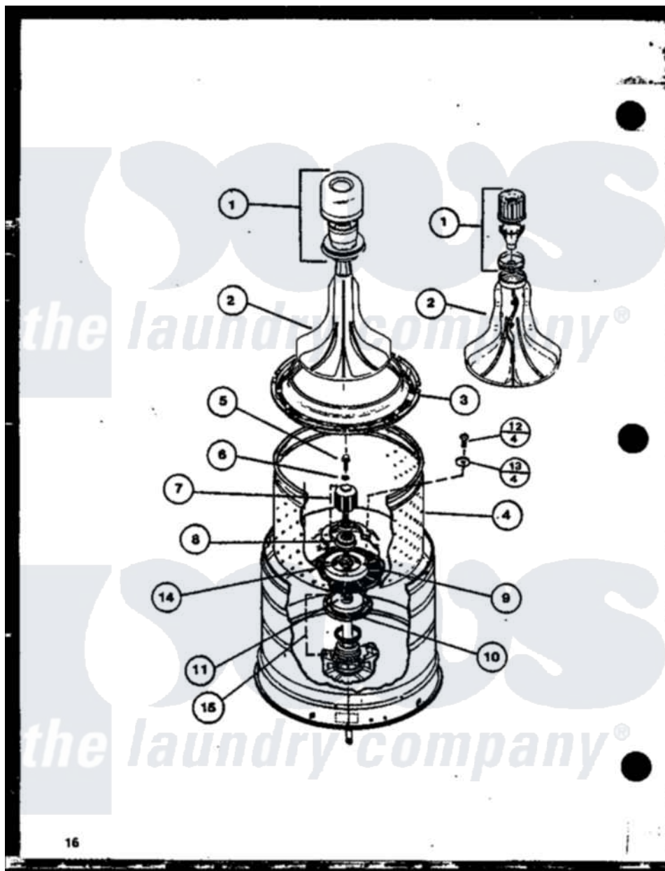
Amana Residential Amana LWD353W (BOM: P1122915W) Washer Parts Parts Diagram 04 - Page 6 Click on the part number to view part
