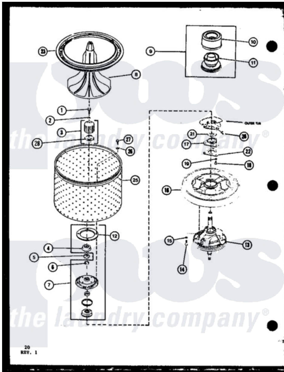
Amana Residential Amana LWD450 (BOM: P7762106W W) Washer Parts Parts Diagram 06 - Page 8 Click on the part number to view part
