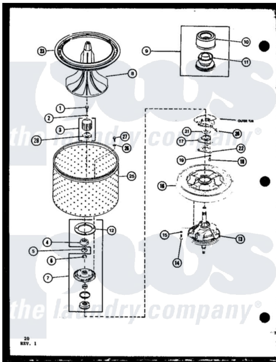
Amana Residential Amana LWD450 (BOM: P7762108W W) Washer Parts Parts Diagram 06 - Page 8 Click on the part number to view part
