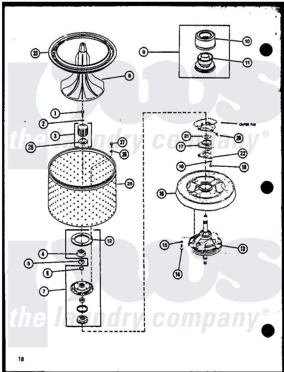
Amana Residential Amana LWD553 (BOM: P7762116W W) Washer Parts Parts Diagram 06 - Page 7 Click on the part number to view part
