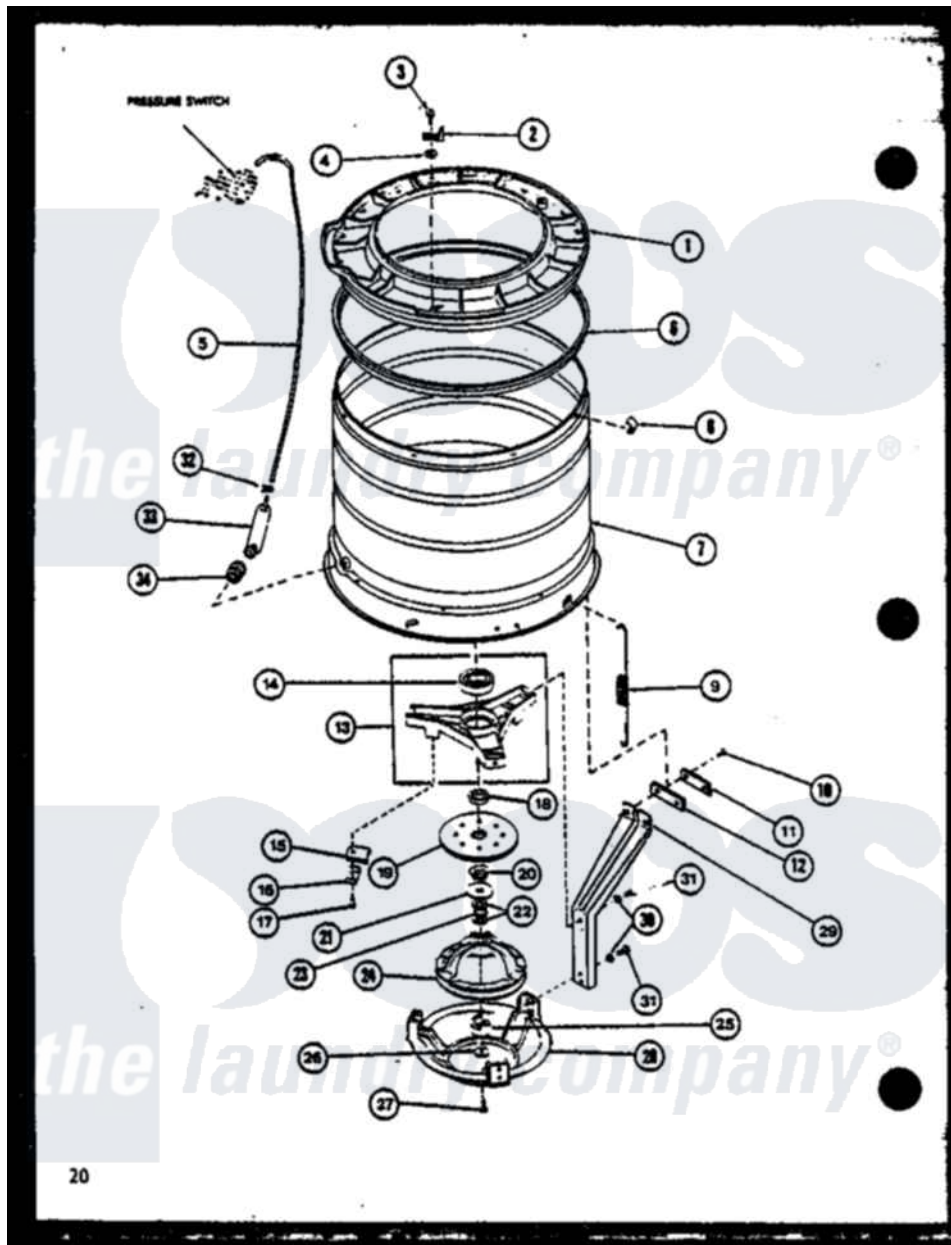
Amana Residential Amana LWD553 (BOM: P7762116W W) Washer Parts Parts Diagram 07 - Page 8 Click on the part number to view part
