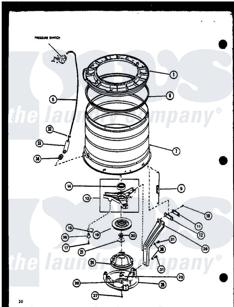
Amana Residential Amana LWD553L (BOM: P1122906W L) Washer Parts Parts Diagram 08 - Page 8 Click on the part number to view part
