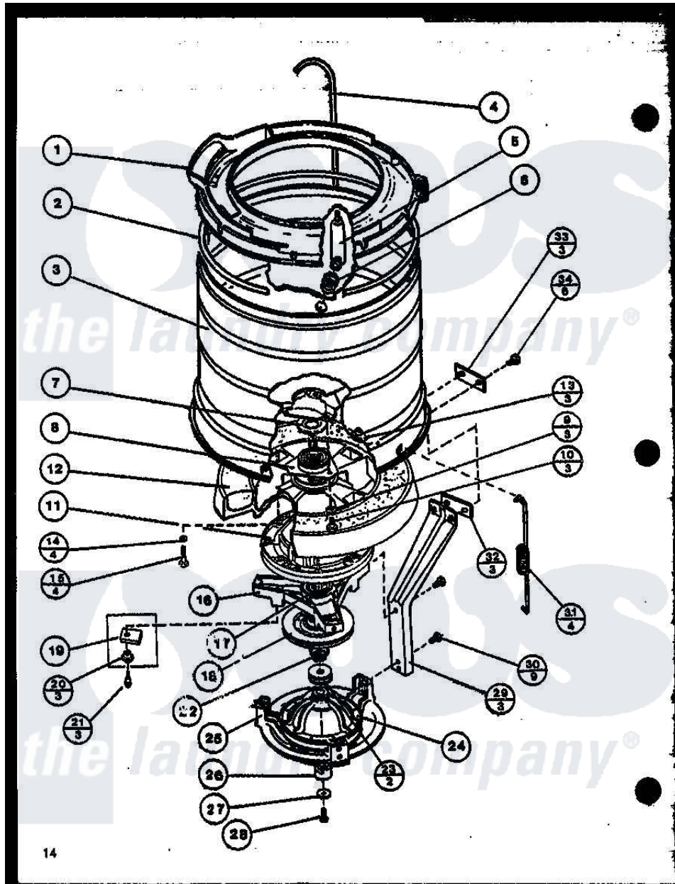
Amana Residential Amana LWD553W (BOM: P1122921W W) Washer Parts Parts Diagram 03 - Page 5 Click on the part number to view part
