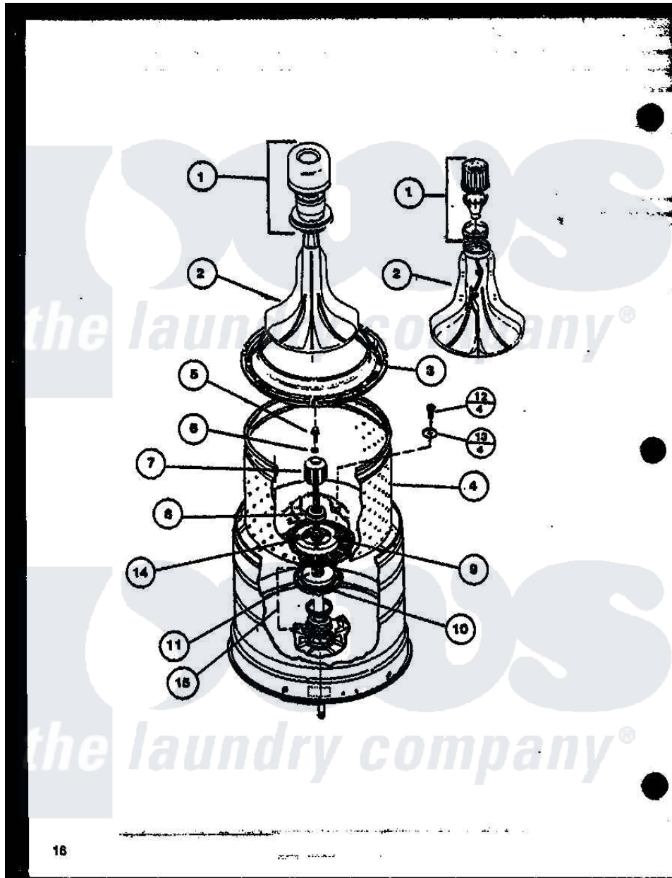
Amana Residential Amana LWD553W (BOM: P1122921W W) Washer Parts Parts Diagram 04 - Page 6 Click on the part number to view part
