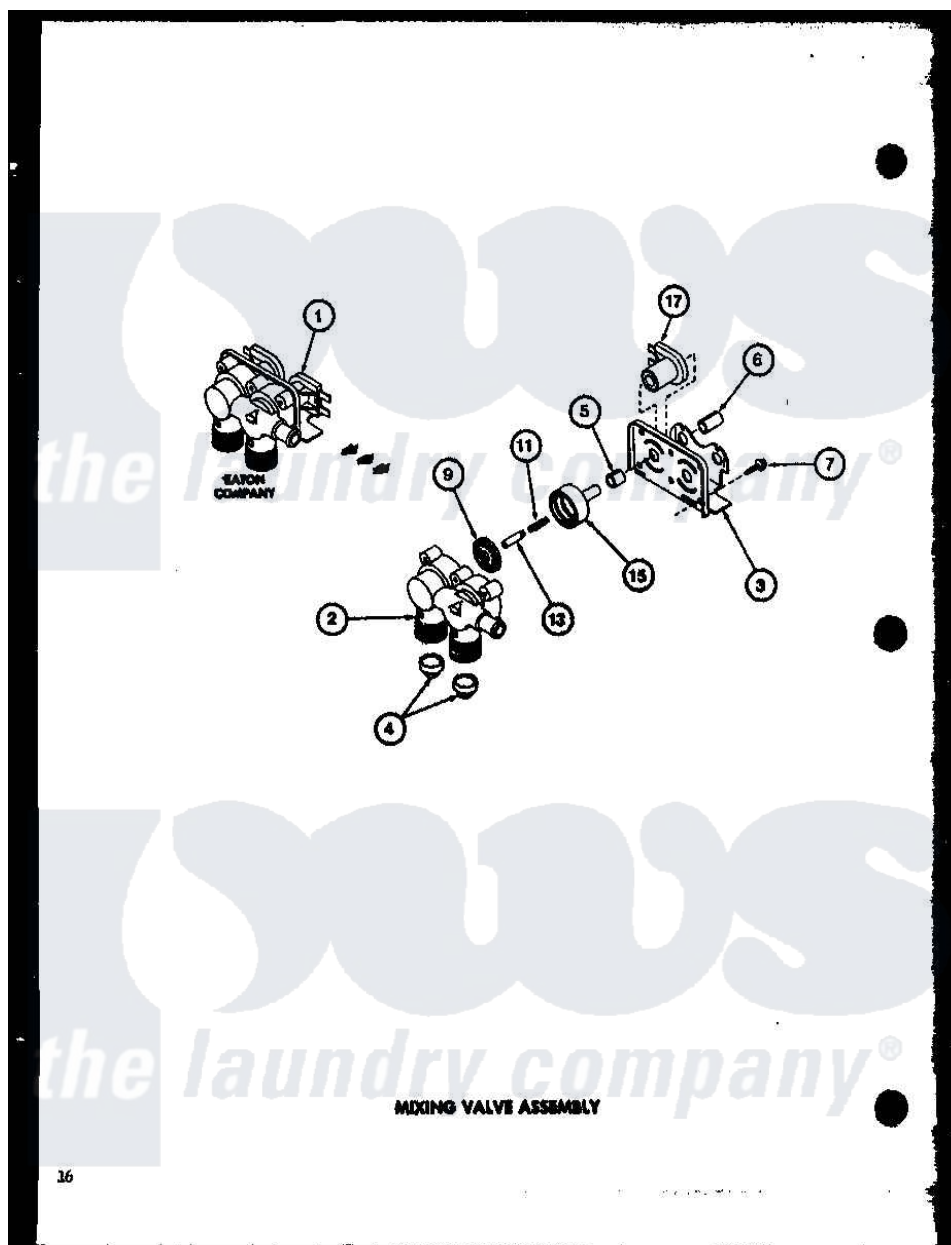
Amana Residential Amana LWD650 (BOM: P7804704W W) Washer Parts Parts Diagram 03 - MIXING VALVE ASSY
