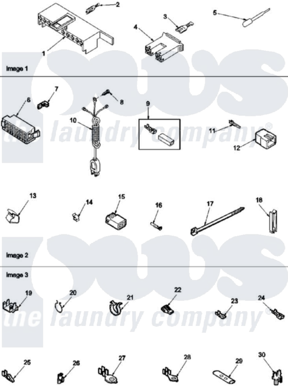
Amana Residential Amana LWD67AL (BOM: PLWD67AL) Washer Parts Parts Diagram 04 - CONNECTION BLOCKS, EXTRACTOR TOOL
