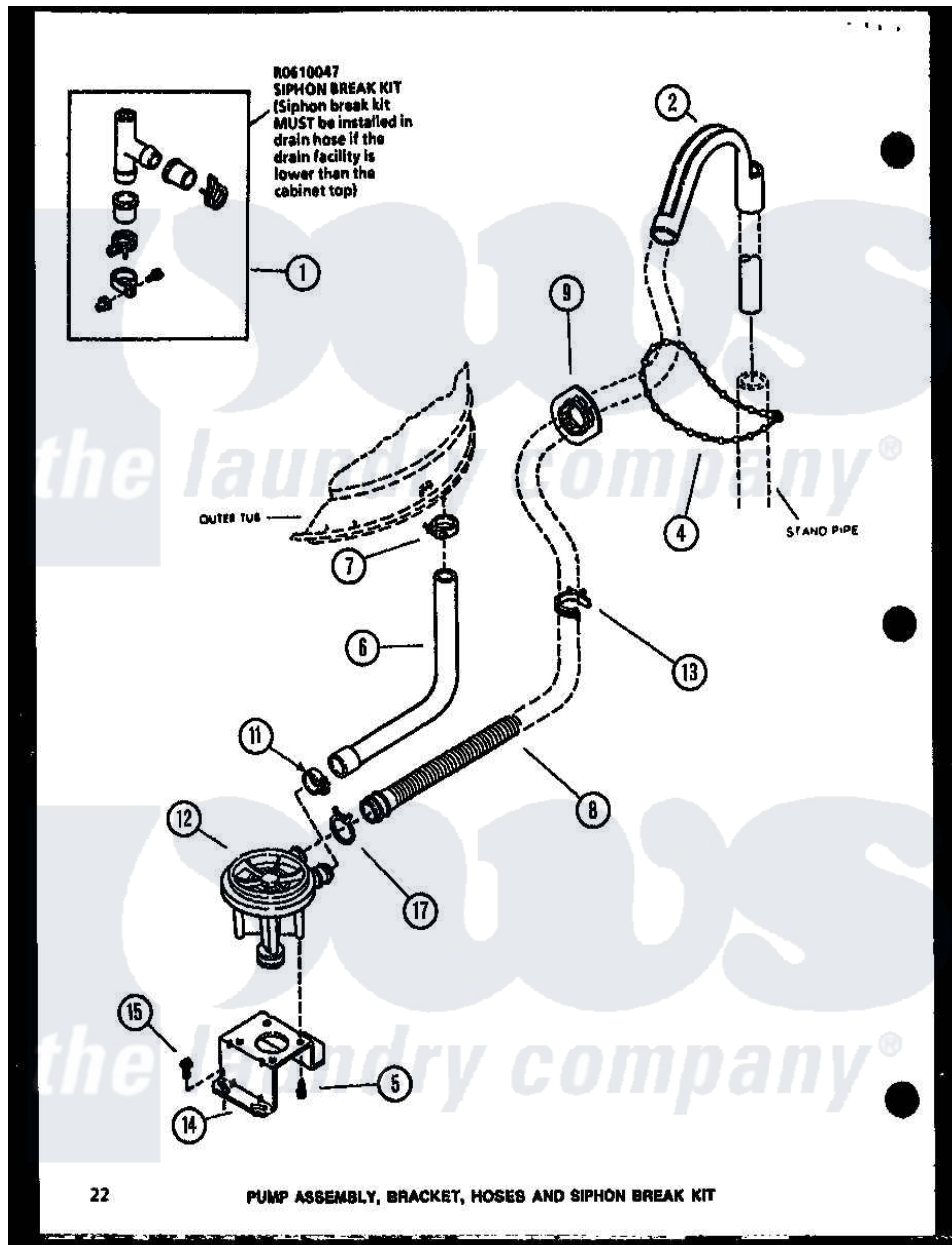
Amana Residential Amana LWD773L (BOM: P1122802W L) Washer Parts Diagram 01 - ASSY Click on the part number to view part
