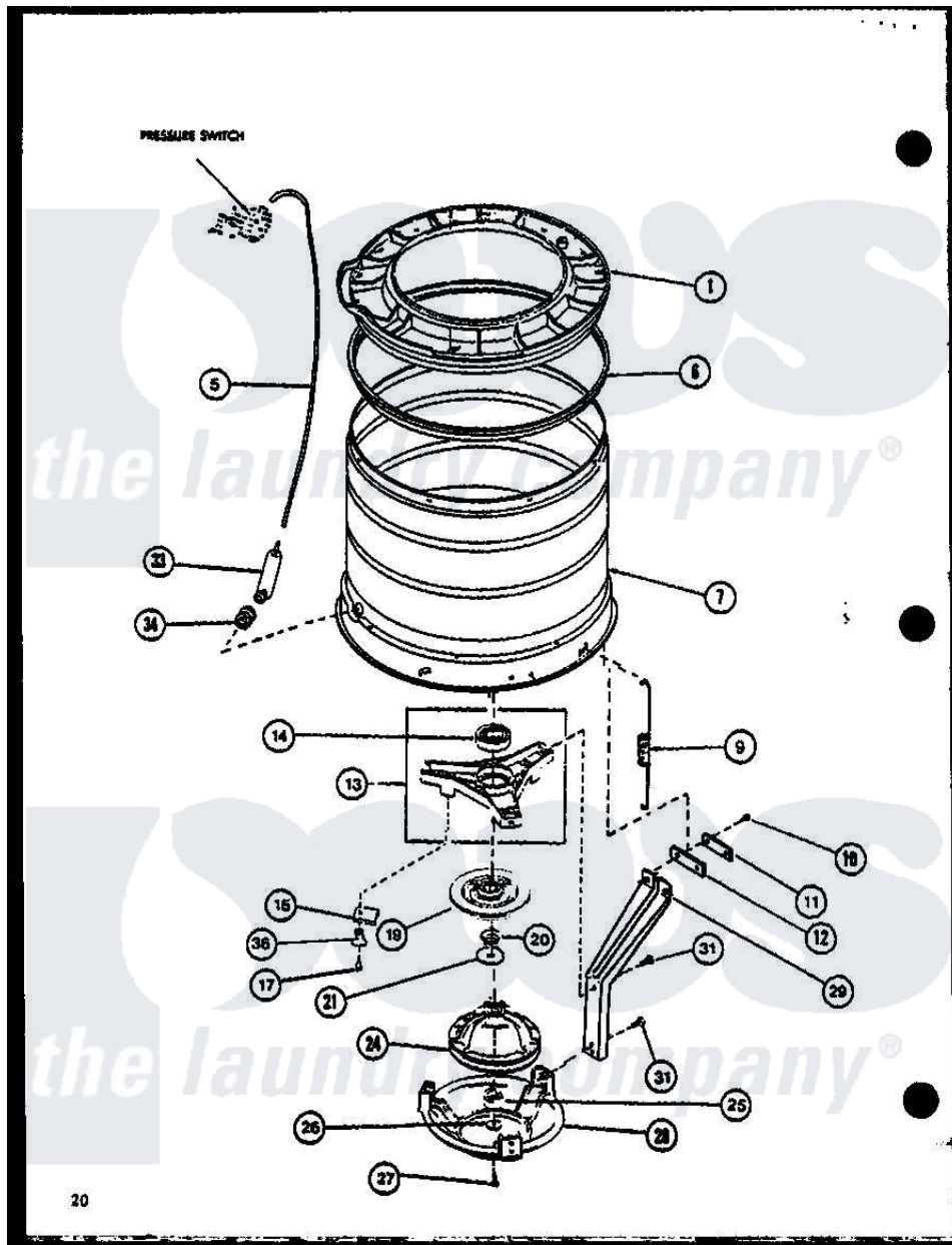
Amana Residential Amana LWD773L (BOM: P1122802W L) Washer Parts Diagram 08 - Page 8 Click on the part number to view part
