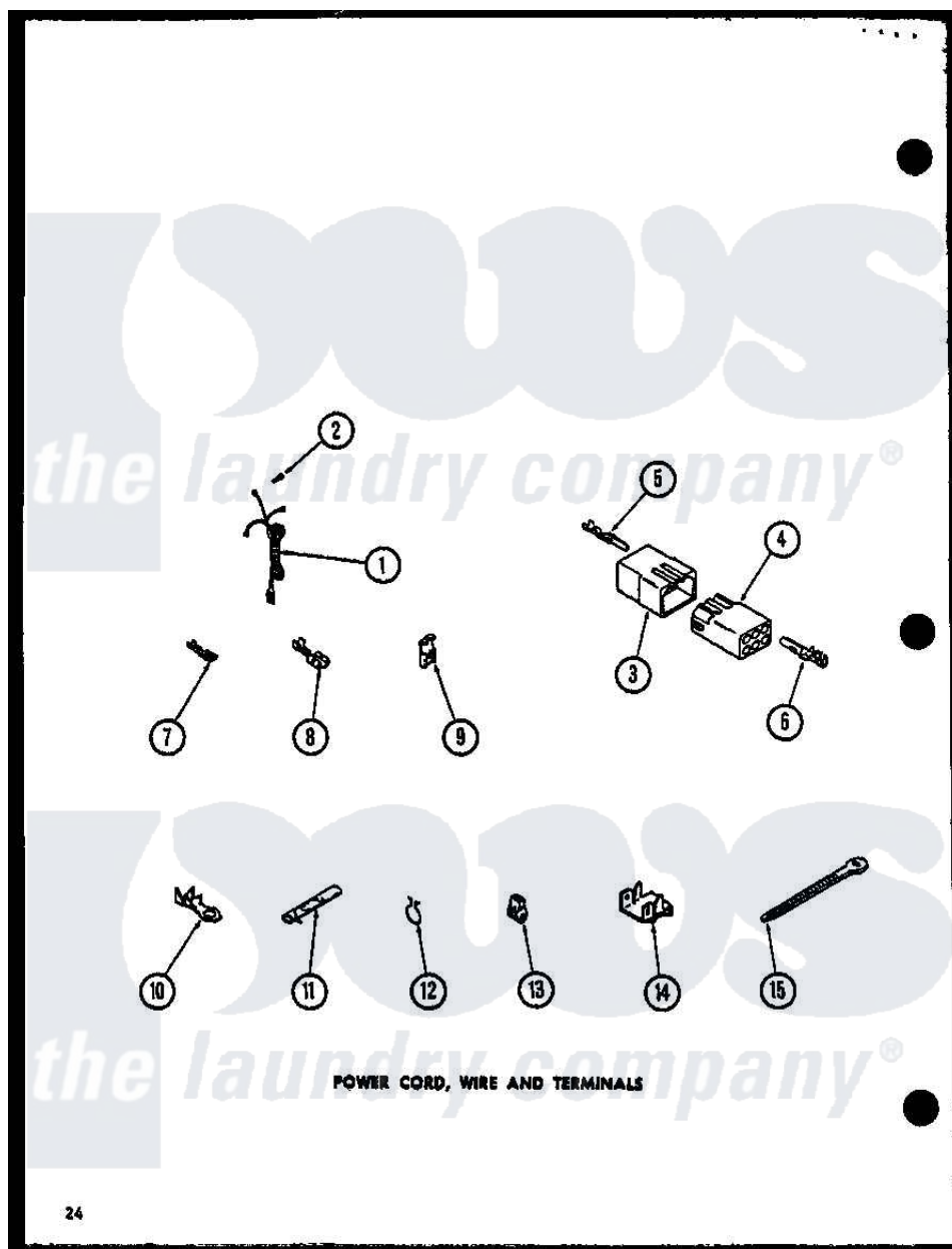
Amana Residential Amana LWD773L (BOM: P1122802W L) Washer Parts Parts Diagram 09 - POWER CORD Click on the part number to view part
