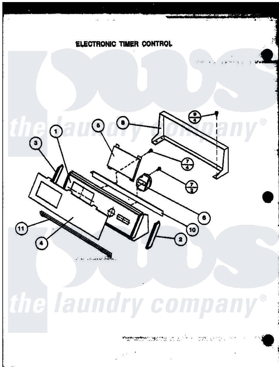
Amana Residential Amana LWD773L (BOM: P1122815W L) Washer Parts Parts Diagram 01 - ELECTRONIC TIMER CONTROL
