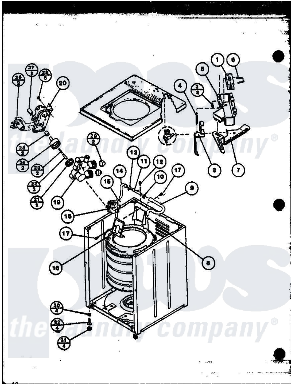
Amana Residential Amana LWD773L (BOM: P1122815W L) Washer Parts Diagram 03 - Page 4 Click on the part number to view part
