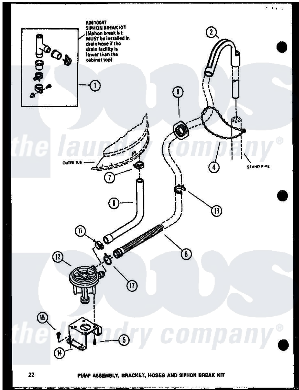
Amana Residential Amana LWD773W (BOM: P1122801W W) Washer Parts Diagram 01 - ASSY Click on the part number to view part
