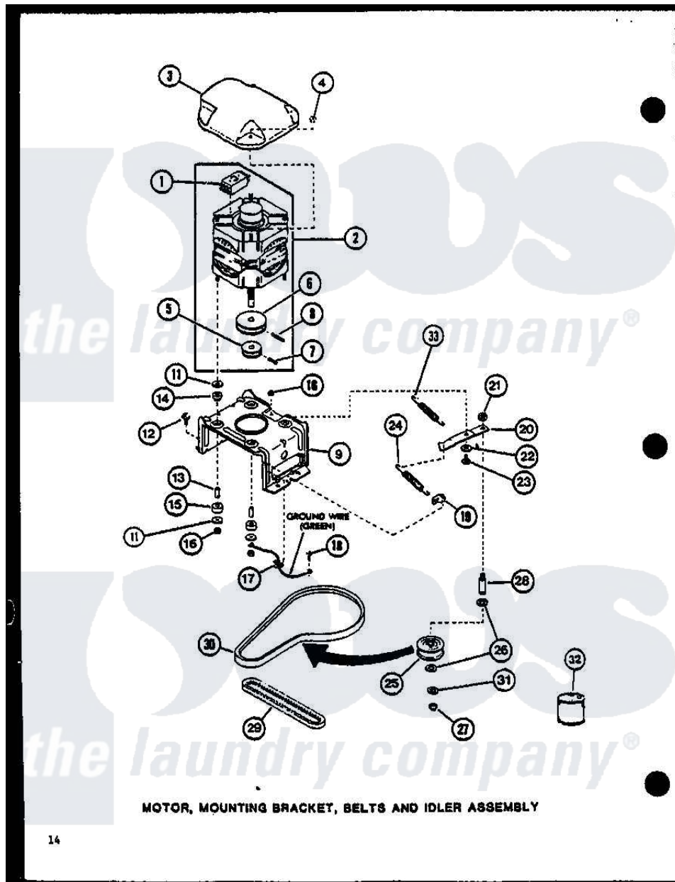
Amana Residential Amana LWD773W (BOM: P1122801W W) Washer Parts Parts Diagram 04 - MOTOR Click on the part number to view part
