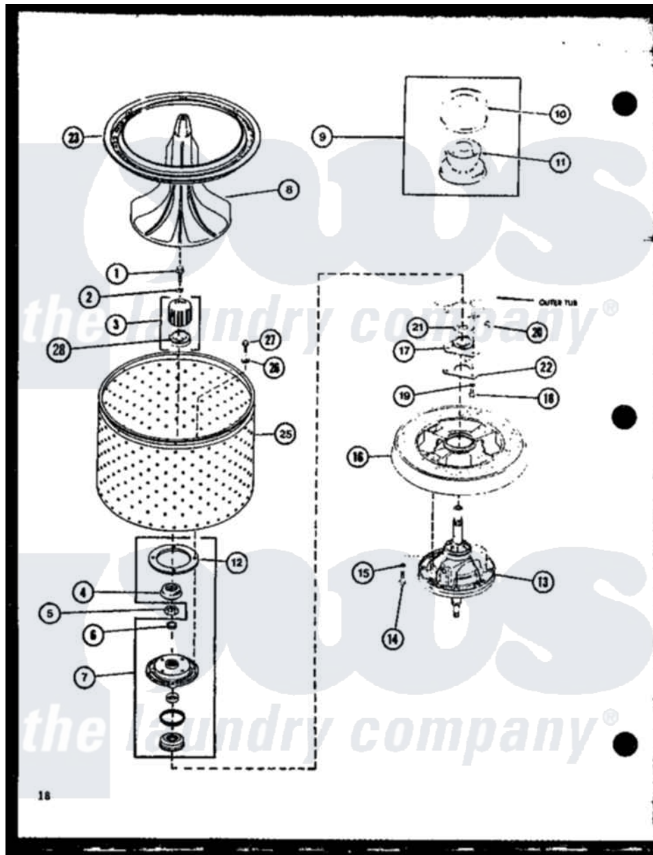
Amana Residential Amana LWD862 (BOM: P7804708W W) Washer Parts Parts Diagram 06 - Page 7 Click on the part number to view part
