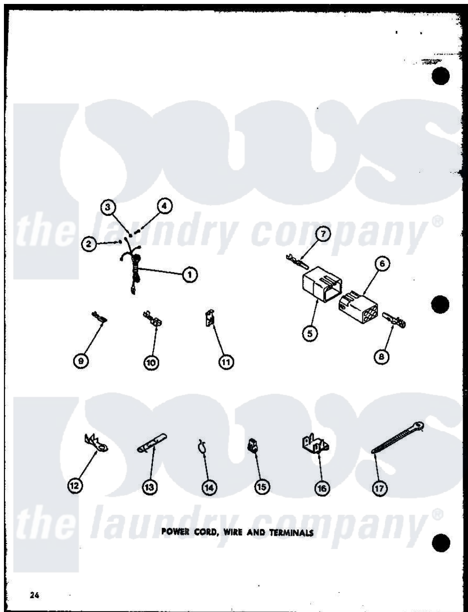
Amana Residential Amana LWD962 (BOM: P7804709W W) Washer Parts Parts Diagram 08 - POWER CORD Click on the part number to view part
