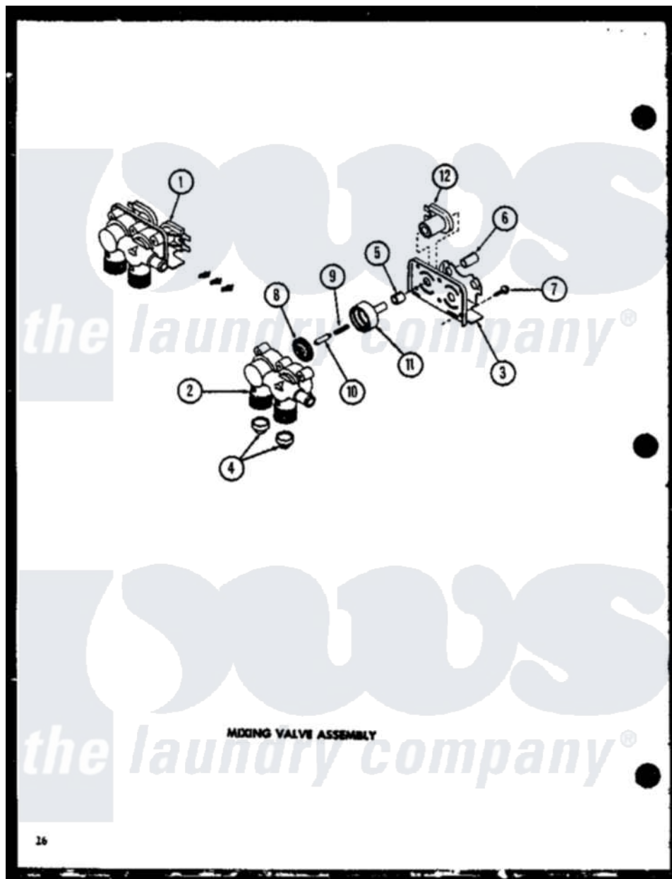
Amana Residential Amana LWD973 (BOM: P1110502W) Washer Parts Parts Diagram 01 - MIXING VALVE ASSY Click on the part number to view part
