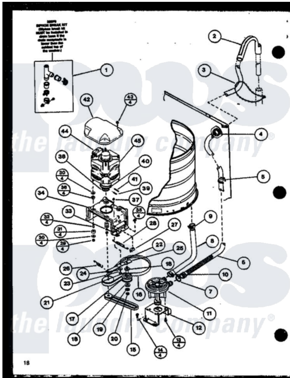
Amana Residential Amana LWD973L (BOM: P1122811W) Washer Parts Parts Diagram 06 - Page 7 Click on the part number to view part
