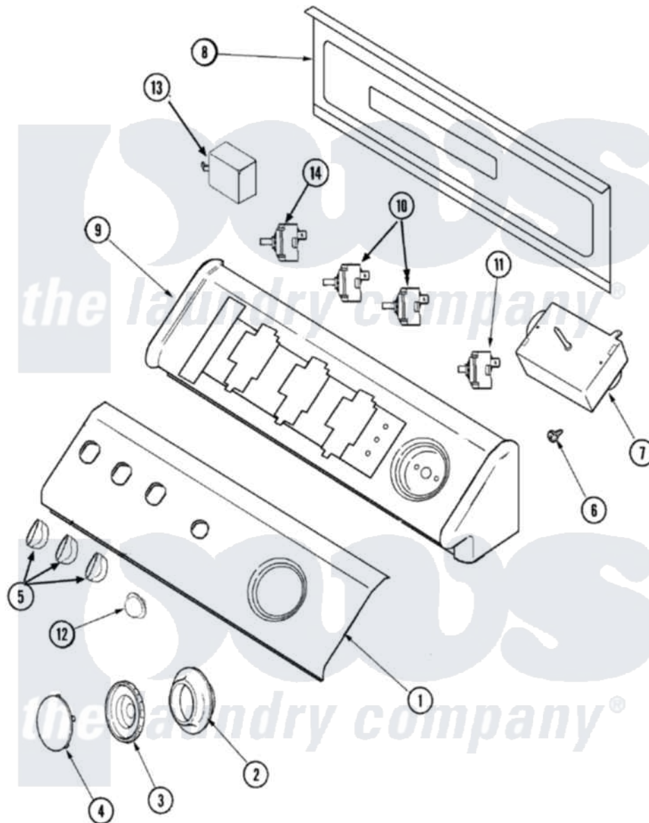
Amana Residential Amana NDE7800AYW Dryer Parts Parts Diagram 02 - CONTROL PANEL Click on the part number to view part
