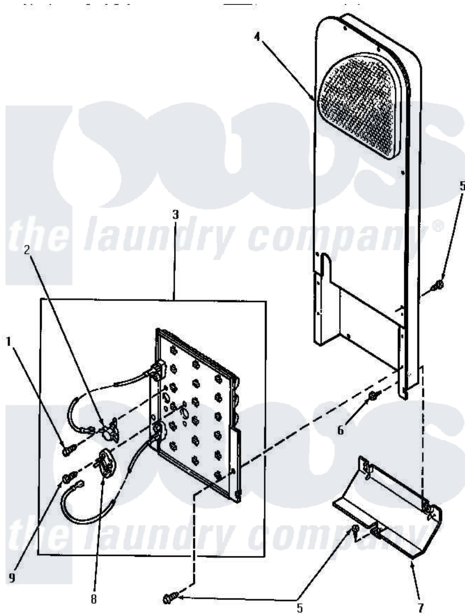
Amana Residential Amana NE8833 Dryer Parts Parts Diagram 05 - HEATER BOX Click on the part number to view part
