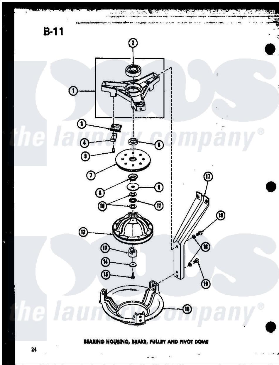
Amana Residential Amana TAA200 (BOM: P7575104W) Washer Parts Parts Diagram 02 - BEARING HOUSING Click on the part number to view part
