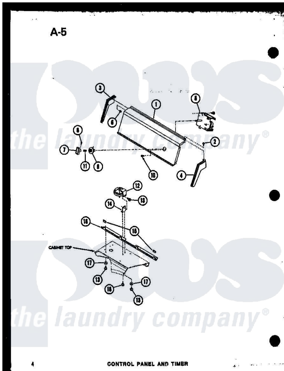
Amana Residential Amana TAA200 (BOM: P7575104W) Washer Parts Parts Diagram 04 - CONTROL PANEL AND TIMER
