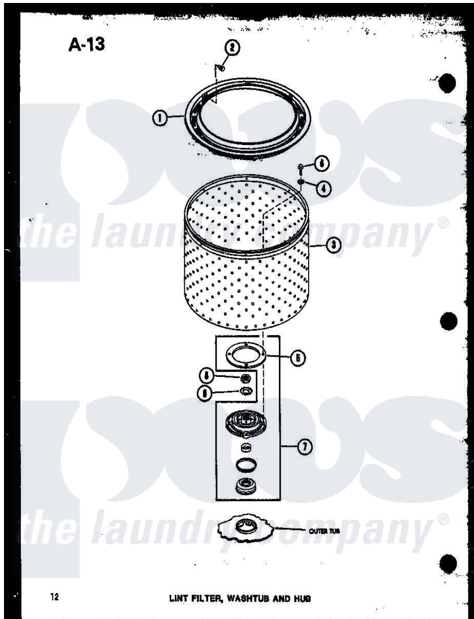
Amana Residential Amana TAA200 (BOM: P7575104W) Washer Parts Parts Diagram 07 - LINT FILTER Click on the part number to view part
