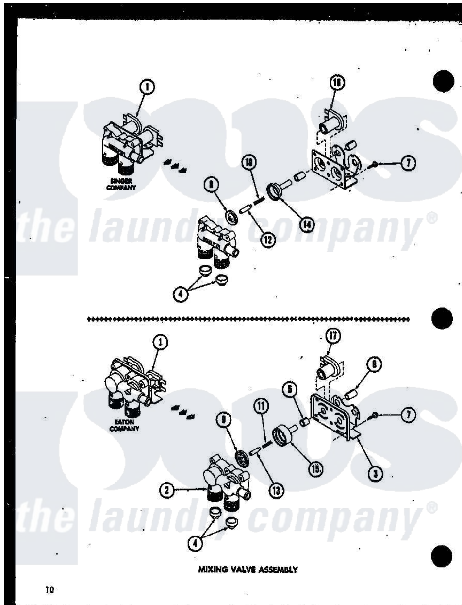
Amana Residential Amana TAA200 (BOM: P7575108W) Washer Parts Parts Diagram 07 - MIXING VALVE ASSY
