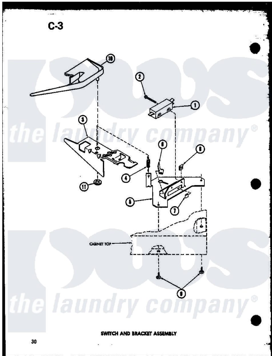
Amana Residential Amana TAA200 (BOM: P7575113W) Washer Parts Diagram 13 - SWITCH AND BRACKET ASSY
