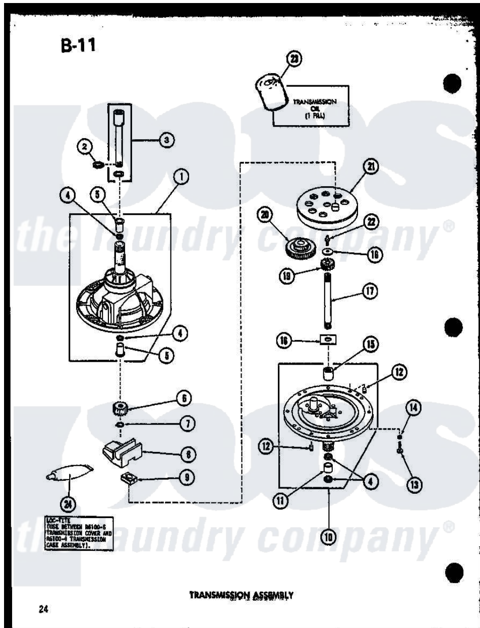
Amana Residential Amana TAA200 (BOM: P7575113W) Washer Parts Diagram 14 - TRANSMISSION ASSY Click on the part number to view part
