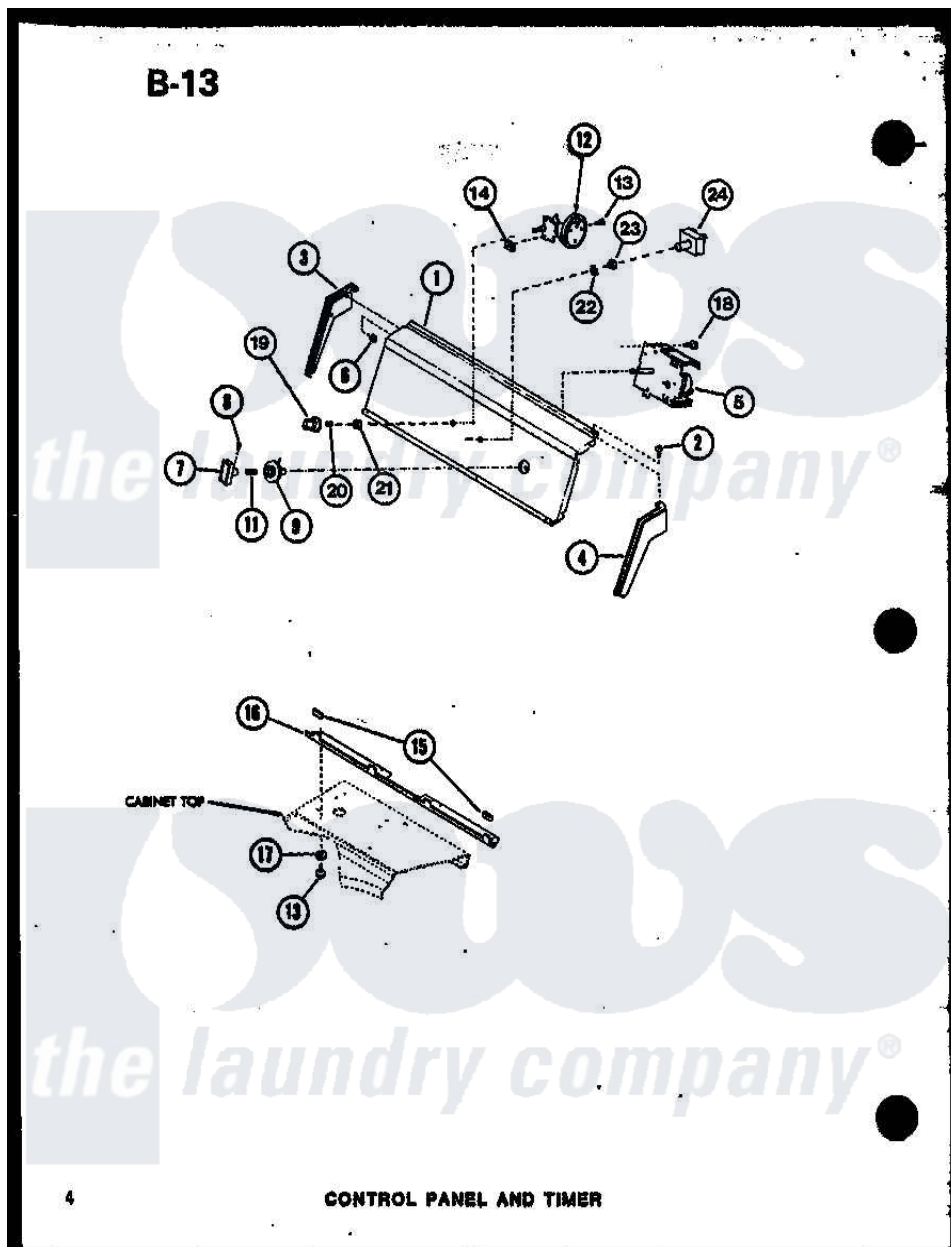
Amana Residential Amana TAA300 (BOM: P7575112W) Washer Parts Parts Diagram 04 - CONTROL PANEL AND TIMER
