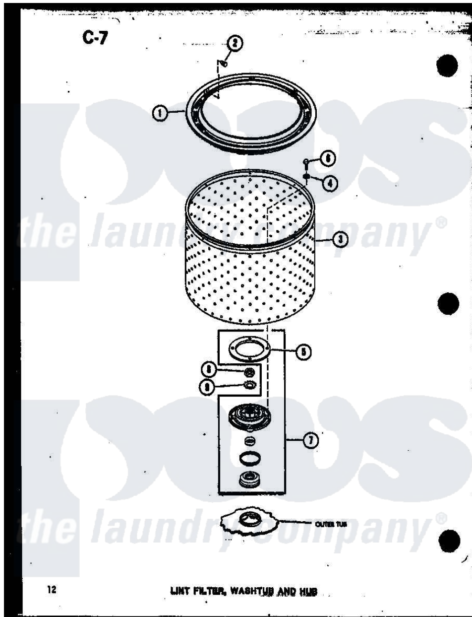
Amana Residential Amana TAA300 (BOM: P7575112W) Washer Parts Parts Diagram 07 - LINT FILTER Click on the part number to view part
