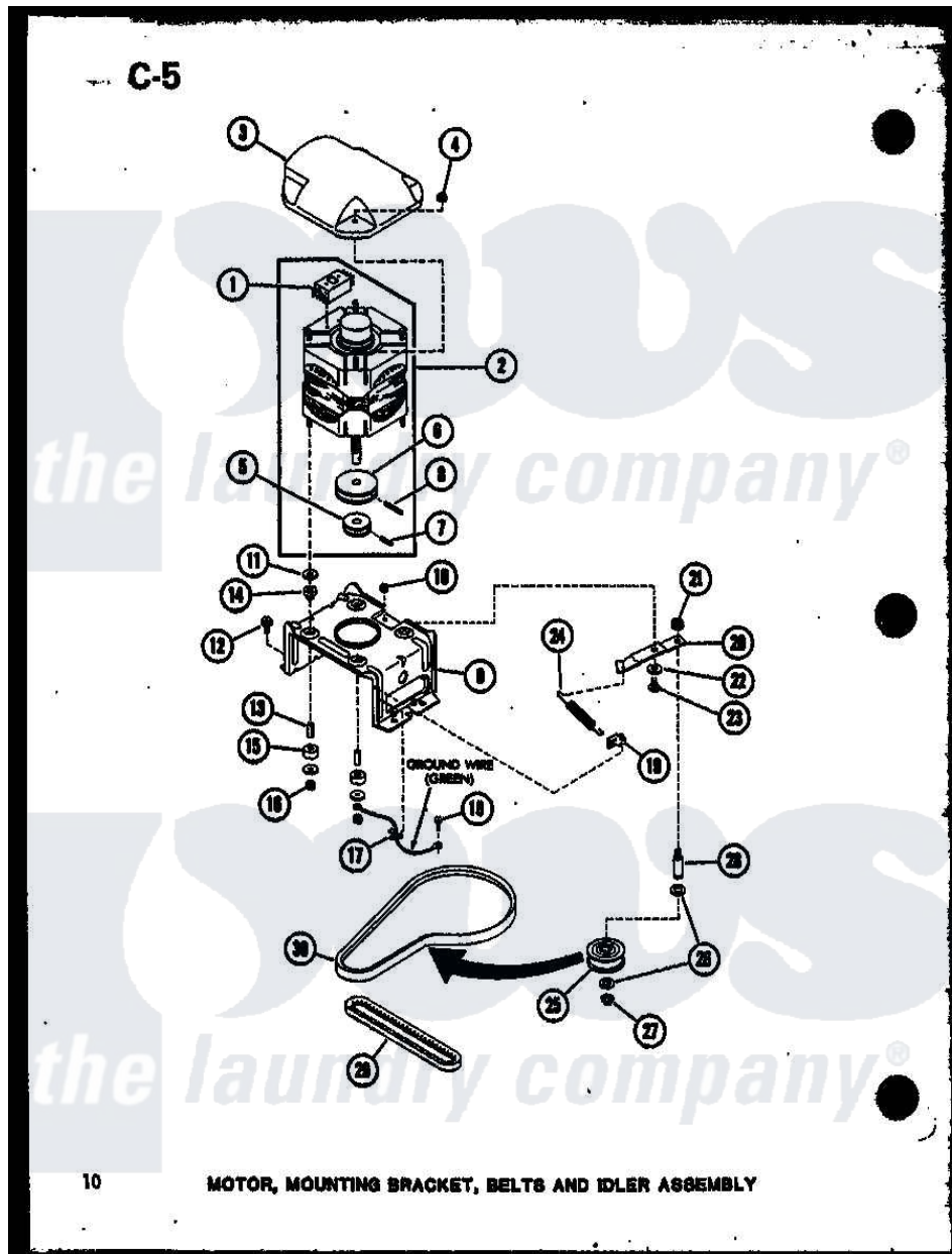
Amana Residential Amana TAA300 (BOM: P7575112W) Washer Parts Parts Diagram 09 - MOTOR Click on the part number to view part
