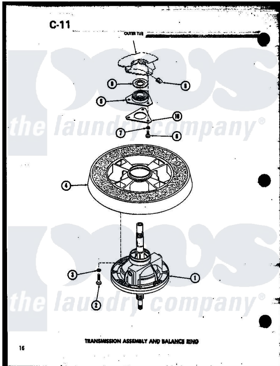
Amana Residential Amana TAA300 (BOM: P7575112W) Washer Parts Parts Diagram 15 - TRANSMISSION ASSY AND BALANCE RING
