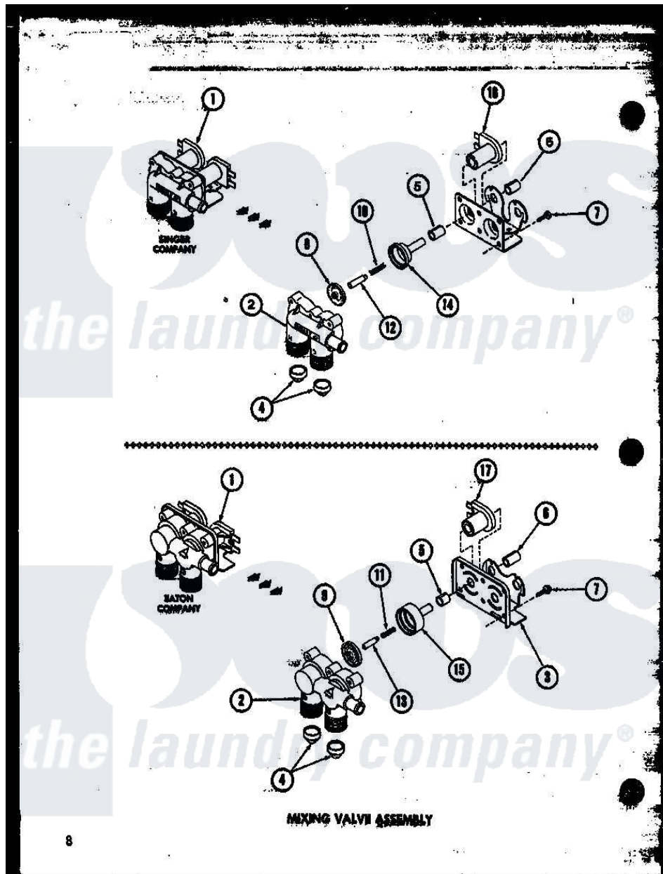
Amana Residential Amana TAA300 (BOM: P7575114W) Washer Parts Parts Diagram 08 - MIXING VALVE ASSY
