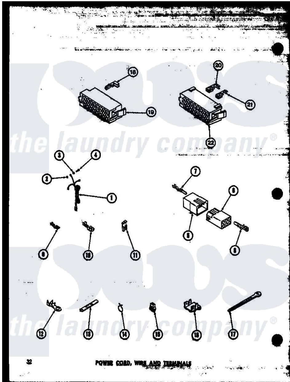
Amana Residential Amana TAA300 (BOM: P7575114W) Washer Parts Parts Diagram 11 - POWER CORD
