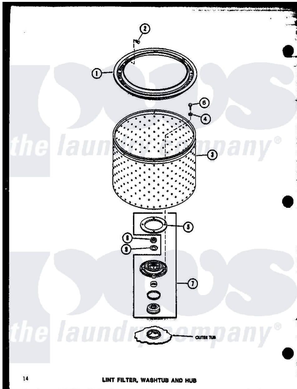
Amana Residential Amana TAA300 (BOM: P7704001W) Washer Parts Parts Diagram 07 - LINT FILTER Click on the part number to view part
