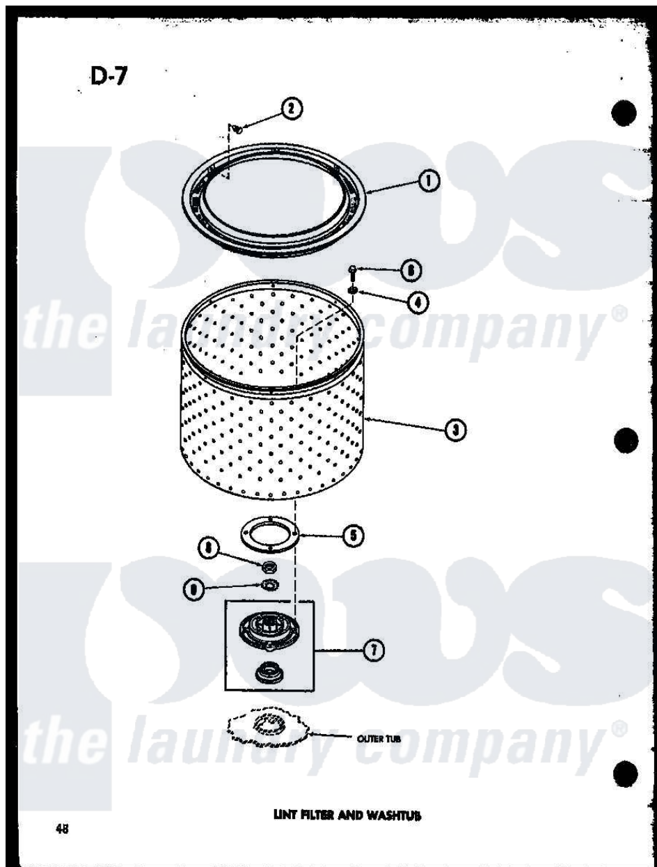
Amana Residential Amana TAA400 (BOM: P7575102W) Washer Parts Parts Diagram 07 - LINT FILTER AND WASHTUB
