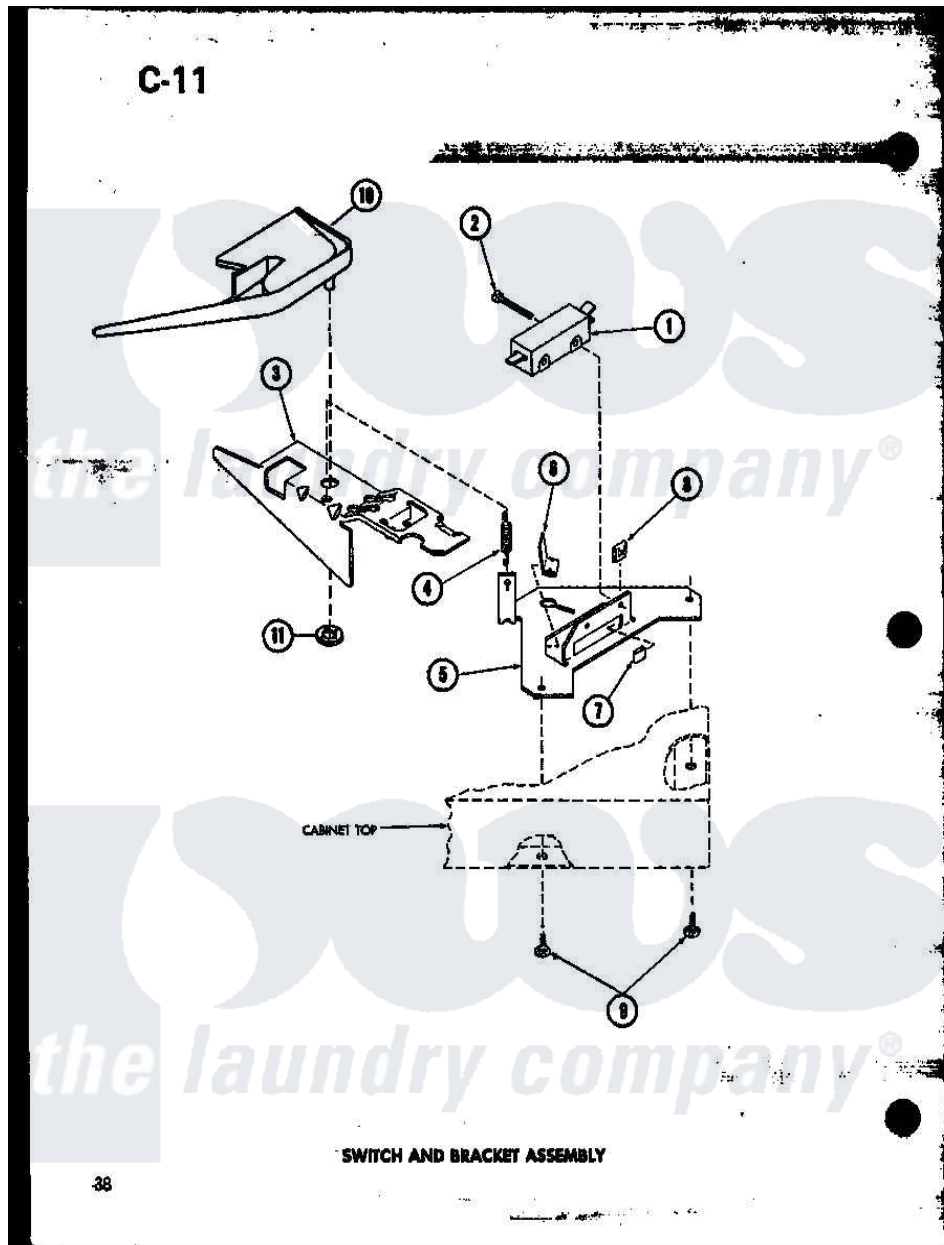
Amana Residential Amana TAA400 (BOM: P7575102W) Washer Parts Parts Diagram 13 - SWITCH AND BRACKET ASSY
