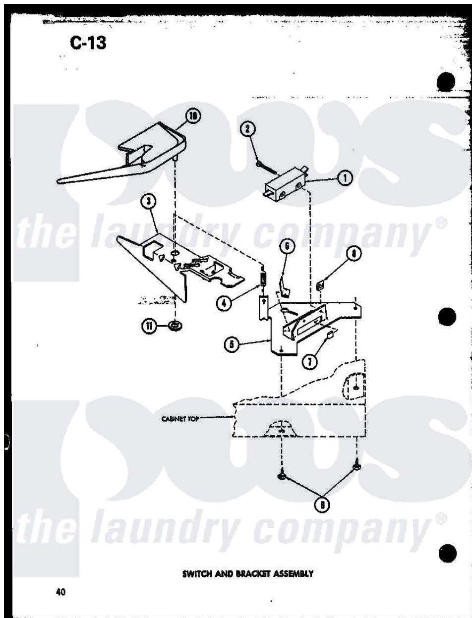
Amana Residential Amana TAA400 (BOM: P7575115W) Washer Parts Diagram 13 - SWITCH AND BRACKET ASSY
