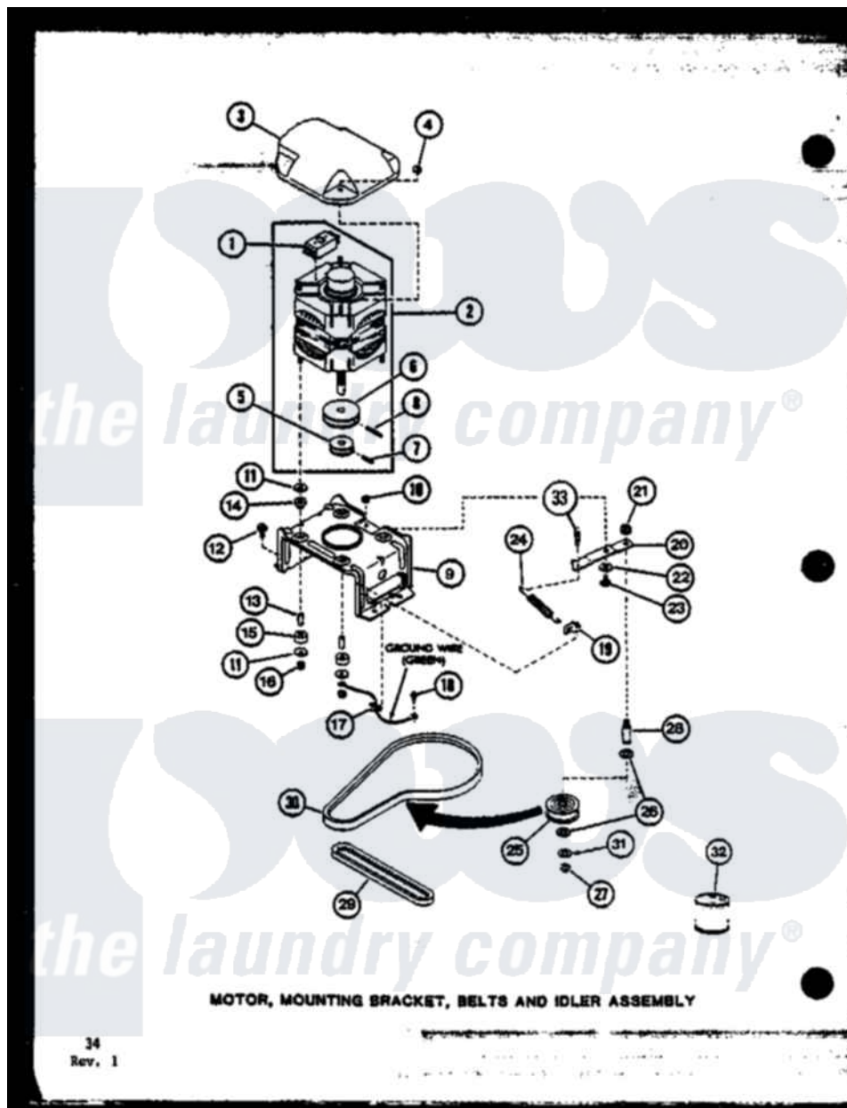
Amana Residential Amana TAA5001 (BOM: P7704008W) Washer Parts Parts Diagram 04 - MOTOR
