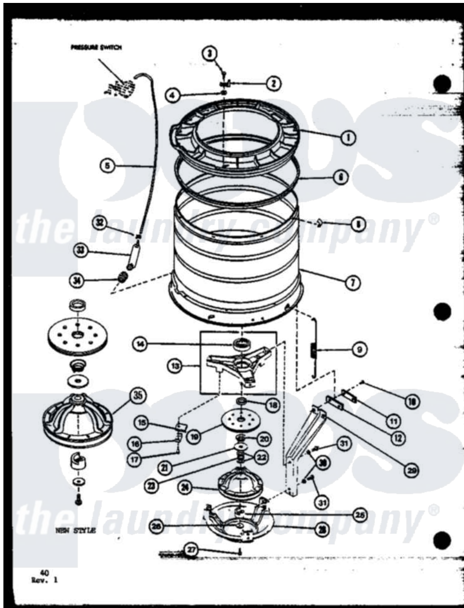
Amana Residential Amana TAA5001 (BOM: P7704008W) Washer Parts Parts Diagram 07 - Page 18 Click on the part number to view part
